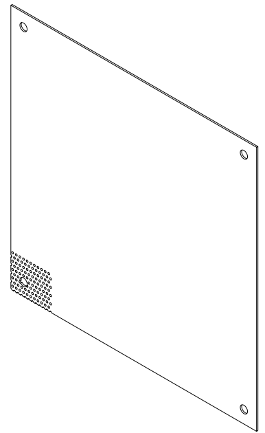
ISOMETRIC VIEW
