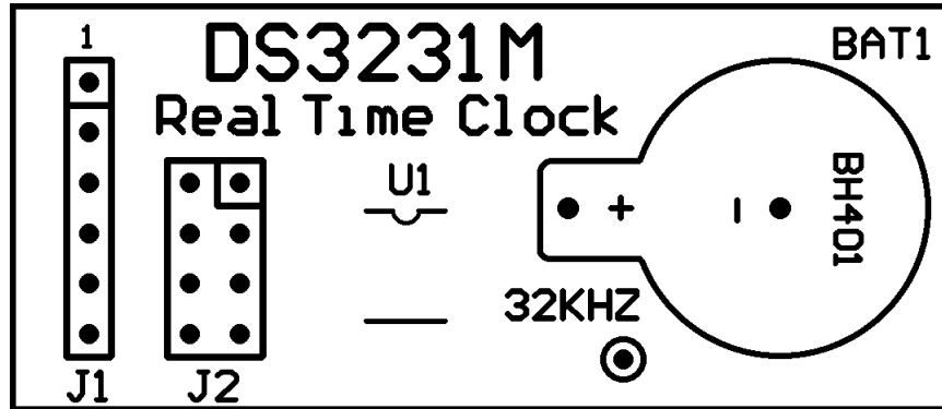
Figure 2. DS3231MPMB1 Peripheral Module Component Placement Guide—Component Side
