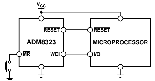
Figure 25. ADM8323 Typical Application Circuit
