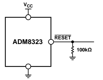
Figure 24. Ensuring \overline{\text{RESET}} Valid to V_{CC} = 0 V
